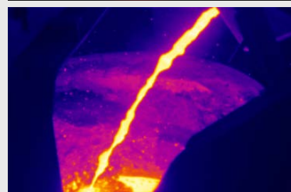
Measurement of casting stream during casting into a mold
