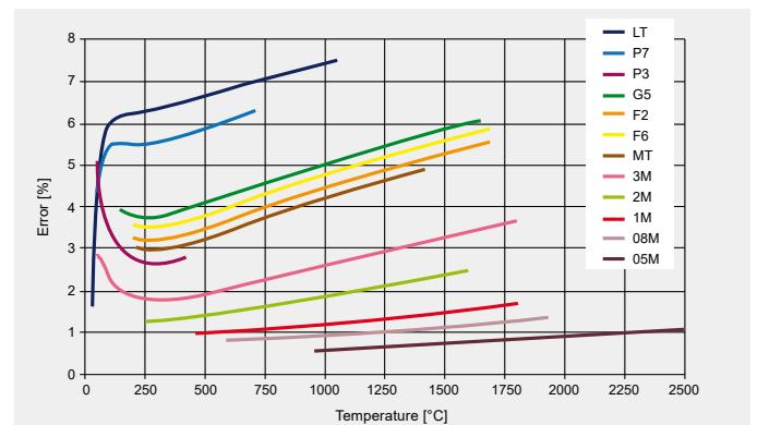
Measuring error in the case of emissivity wrongly adjusted by 10% as a function of the wavelength and object temperature (LT: 8 - 14 \mu\text{m} ; P7: 7.9 \mu\text{m} ; P3: 3.43 \mu\text{m} ; G5: 5 \mu\text{m} ; MT: 3.9 \mu\text{m} ; F2: 4.24 \mu\text{m} ; F6: 4.64 \mu\text{m} ; 3M: 2.3 \mu\text{m} ; 2M: 1.6 \mu\text{m} ; 1M: 1.0 \mu\text{m} ; 08M: 800 nm; 05M: 525 nm)
