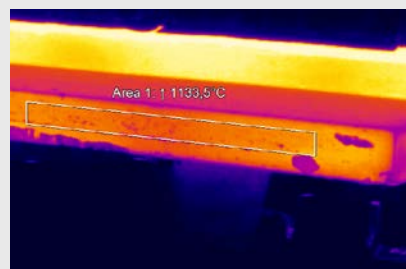
Run-off area of a continuous casting plant
